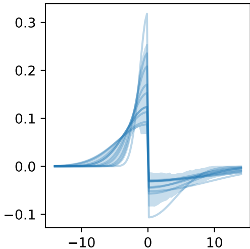
event=PyData-Berlin
